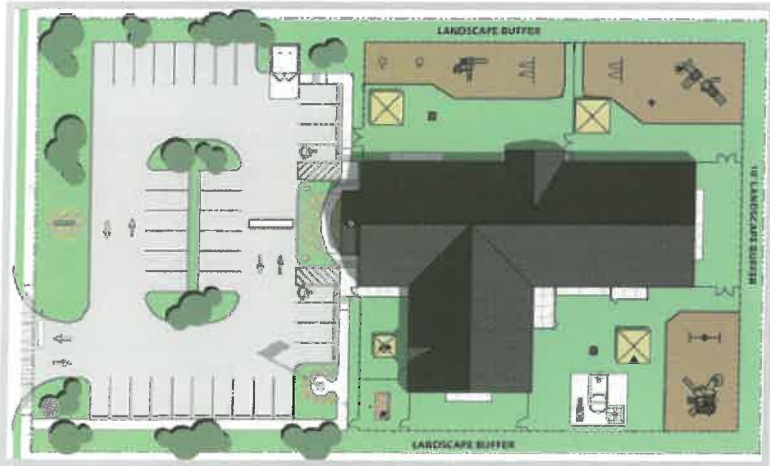
Prototypical Site Plan 60,000 sf site, 12,000 sf building
